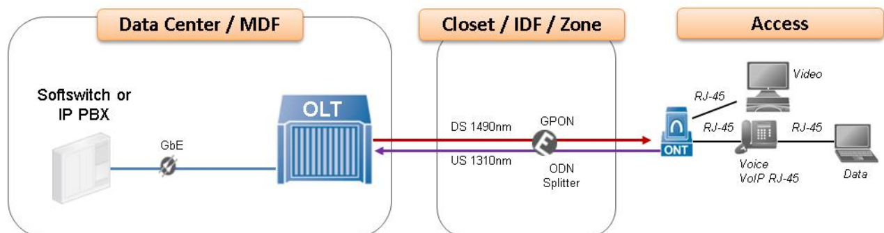
Figure 2: VoIP over Optical LAN architecture
