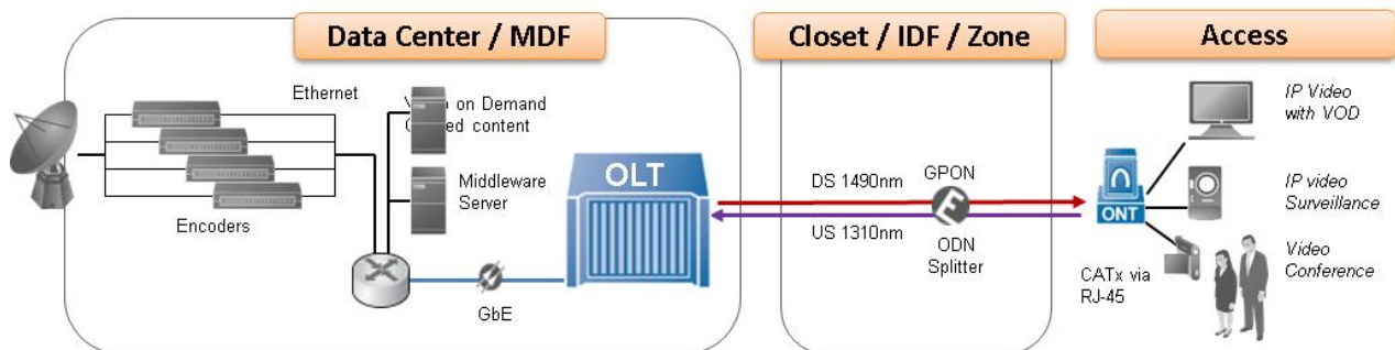
Figure 4: IP video over Optical LAN architecture
