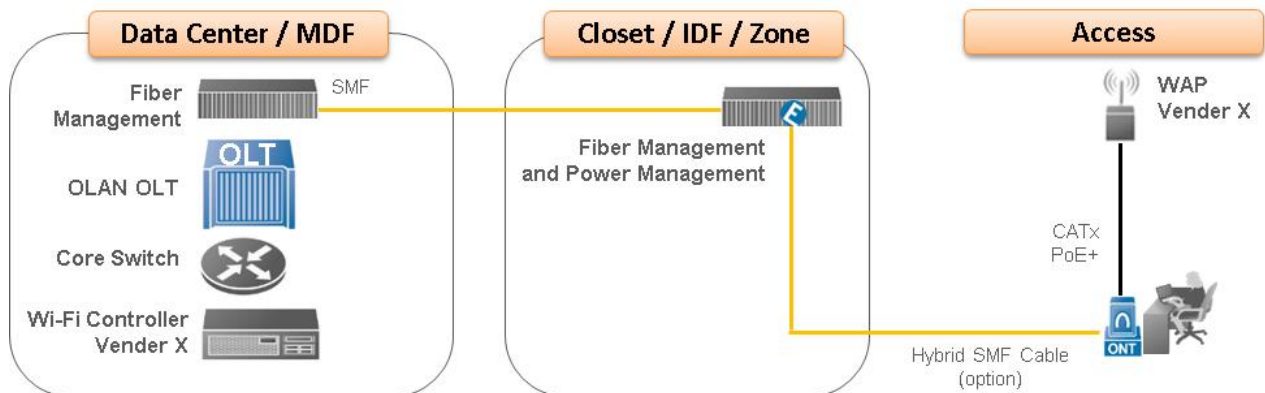
Figure 6: Wi-Fi over Optical LAN architecture
