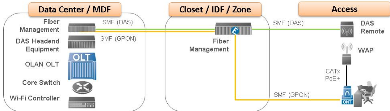
Figure 7: DAS over fiber with synergies with Optical LAN architecture
