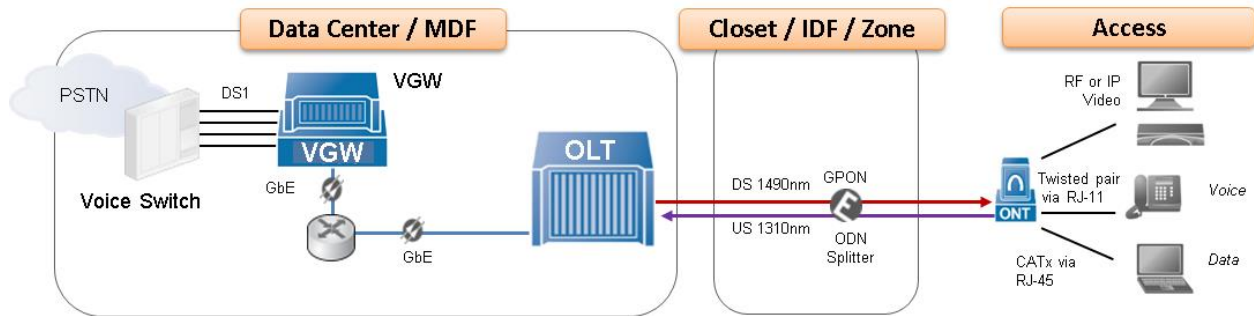
Figure 3: Analog (POTS) over Optical LAN architecture
