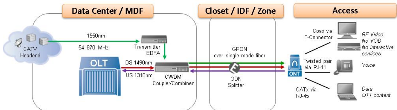
Figure 5: RF video over Optical LAN architecture
